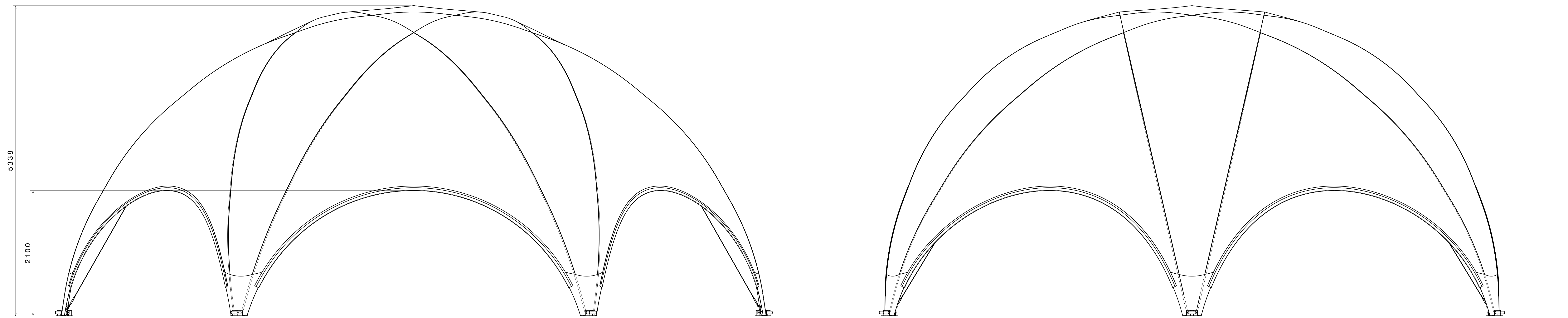
Auxiliary view A
